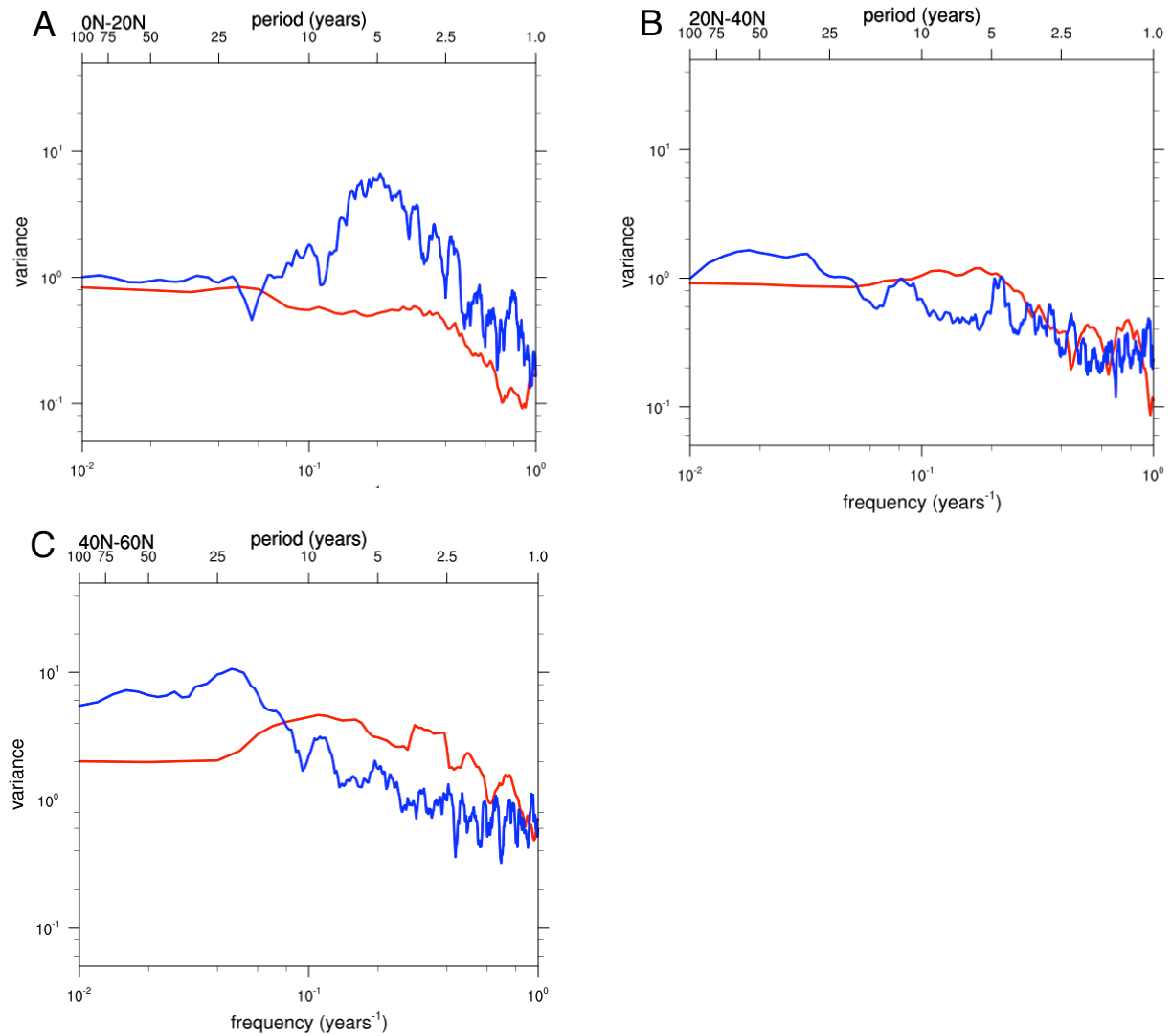
Figure S2: Power spectra of North Atlantic SST (0°-80°W) from the GFDL_CM2_1 model in different latitude bands (A) 0°-20°N; (B) 20°N-40°N; (C) 40°N-60°N. The blue lines are from the 500-year pre-industrial simulation with the fully coupled model, and the red lines are from the 100-year pre-industrial slab-ocean version of the model.
